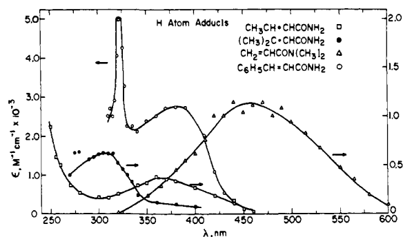
Figure 11. Spectra formed by reaction of H atoms with 1 mM crotonamide, \beta,\beta -dimethylacrylamide, N,N -dimethylacrylamide, and cinnamamide in 1 M aqueous t -BuOH at pH 1.0 ( \text{HClO}_4 ) under Ar. Total dose 8–19 krad/pulse.
