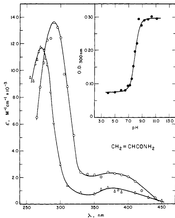
Figure 1. Initial transient absorption spectra produced by reaction of e_{\text{aq}}^- with 2 mM acrylamide at pH 9.2 (O) and 4.0 ( \Delta ) in 1.0 M aqueous t -BuOH under Ar (1 atm). Total dose 4 krad/pulse; absorbance measured \sim 0.2 \mu\text{sec} after the pulse. Insert: change in absorbance at 300 nm with pH.
