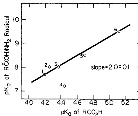
Figure 13. Correlation of pK_a of protonated electron adducts of unsaturated amides \dot{R}C(OH)NH_2 with pK_a of corresponding RCO_2H . R: 1, C_6H_5 ; 2, CH_2CH ; 3, CH_2CCH_3 ; 4, trans - C_6H_5CHCH ; 5, trans - CH_3CHCH ; 6, (CH_3)_2CCH .
