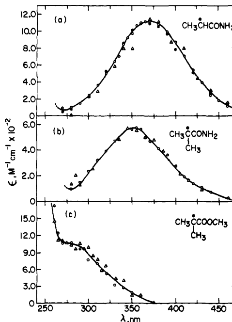
Figure 9. (a) Absorption spectrum of the radical CH_3\dot{C}HCONH_2 ; formed according to eq 9 ( \bullet ); normalized transient spectrum measured 35 \mu sec after the reaction of e_{aq}^- with 0.5 mM acrylamide at pH 9.8 in 0.25 M aqueous t -BuOH under Ar ( \Delta ); transient spectrum from the reaction of H atoms with 2 mM acrylamide (O) at pH 0.9 and in 1.0 M aqueous t -BuOH under Ar. (b) Secondary transient absorption spectrum produced by decay of electron adduct of 2 mM methacrylamide in 1.0 M aqueous t -BuOH at pH 10.0 ( \Delta ); spectrum produced by reaction of H atoms with 3 mM methacrylamide in 1.0 M aqueous t -BuOH at pH 0.9 under Ar (O); total dose 19 krads/pulse. (c) Transient absorption spectrum produced by the reaction of H atoms with 0.5 mM methyl methacrylate in 0.4 M aqueous t -BuOH at pH 1.0 under Ar (O); secondary transient absorption spectrum produced by reaction of e_{aq}^- with 0.5 mM methylmethacrylate in 0.4 M aqueous t -BuOH at pH 9.4 under Ar ( \Delta ); total dose 4 krads/pulse.
