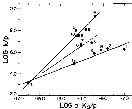
Figure 10. Brønsted correlation of catalytic rate constants for \beta -protonation of acrylamide anion radical: 1, H_2PO_4^- ; 2, NH_4^+ ; 3, +H_3NCH_2CO_2^- ; 4, (CH_3)_3NH^+ ; 5, HCO_3^- ; 6, c-C_6H_{11}NH_3^+ ; 7, C_2H_5NH_3^+ ; 8, (C_2H_5)_3NH^+ ; 9, (C_2H_5)_2NH_2^+ ; 10, c-C_5H_{10}NH_2^+ ; 11, c-C_4H_9NH_2^+ ; 12, HPO_4^{2-} ; 13, H_2O ; 14, B(OH)_3
